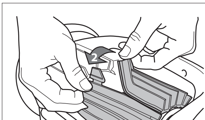
Figure 25. Undo the Tabs of the Brush
